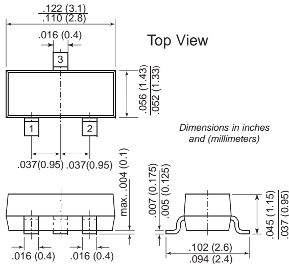
TO-236AB (SOT-23)
